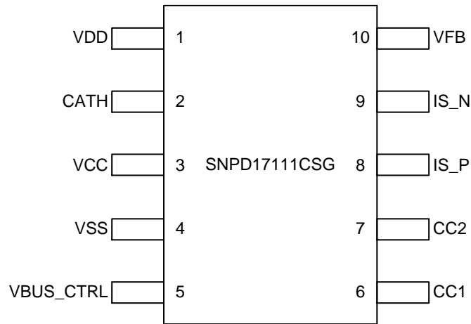
Figure 2–2 SNPD17111CSG Pin Assignment
