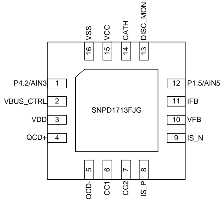
Figure 2-10 SNPD1713FJG Pin Assignment
