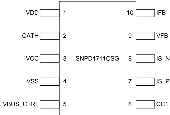
Figure 2-1 SNPD1711CSG Pin Assignment
