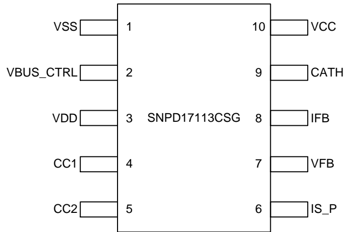
Figure 2–4 SNPD17113CSG Pin Assignment
