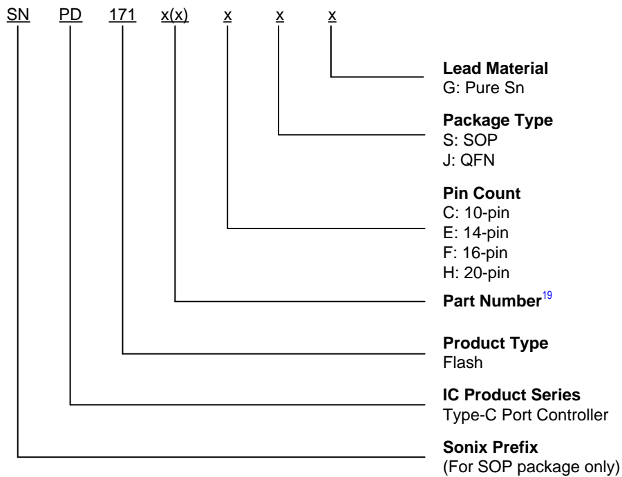
Figure 6–1 Device Nomenclature
