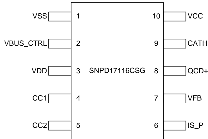
Figure 2–6 SNPD17116CSG Pin Assignment
