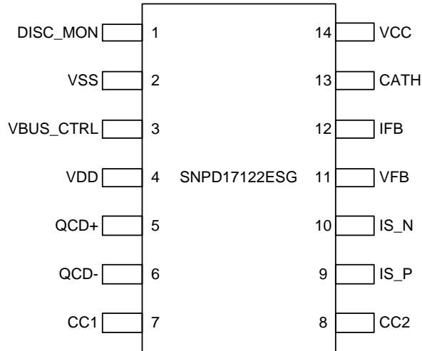
Figure 2-9 SNPD17122ESG Pin Assignment
