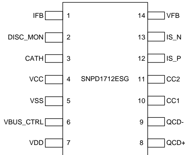
Figure 2-7 SNPD1712ESG Pin Assignment
