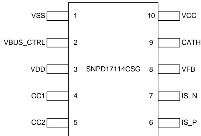
Figure 2-5 SNPD17114CSG Pin Assignment
