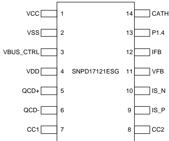
Figure 2-8 SNPD17121ESG Pin Assignment
