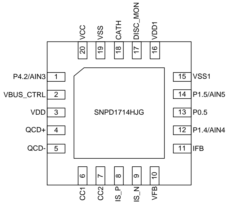
Figure 2-12 SNPD1714HJG Pin Assignment
