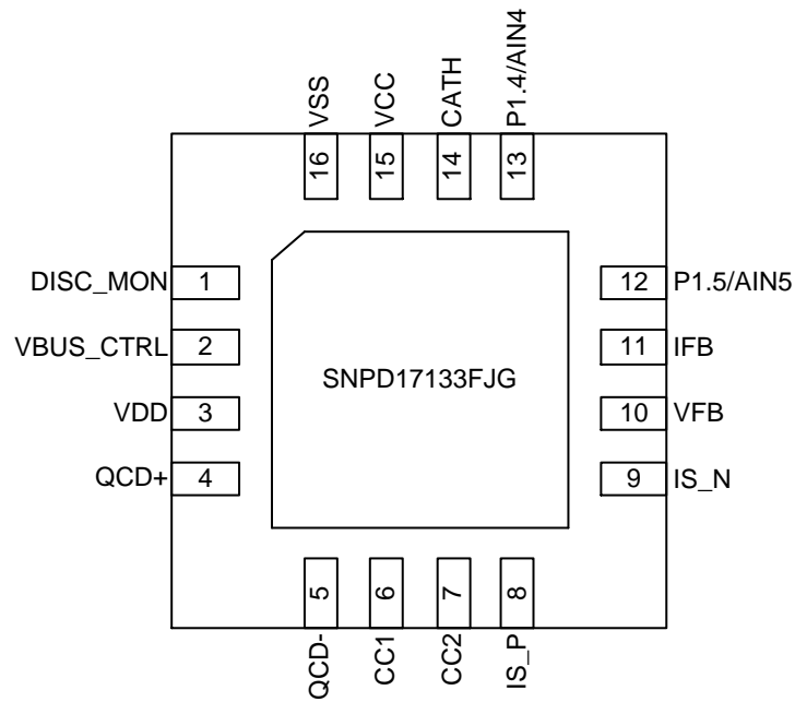
Figure 2-11 SNPD17133FJG Pin Assignment
