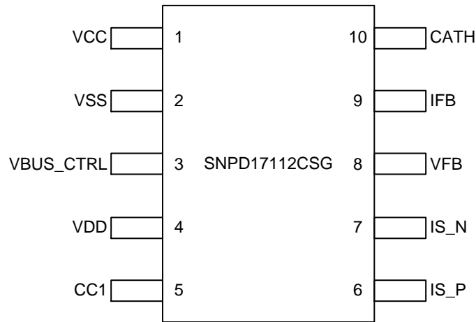
Figure 2–3 SNPD17112CSG Pin Assignment
